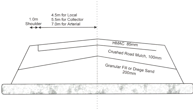
Figure 6 Typical Road Section for Estimating Aggregate Usage
